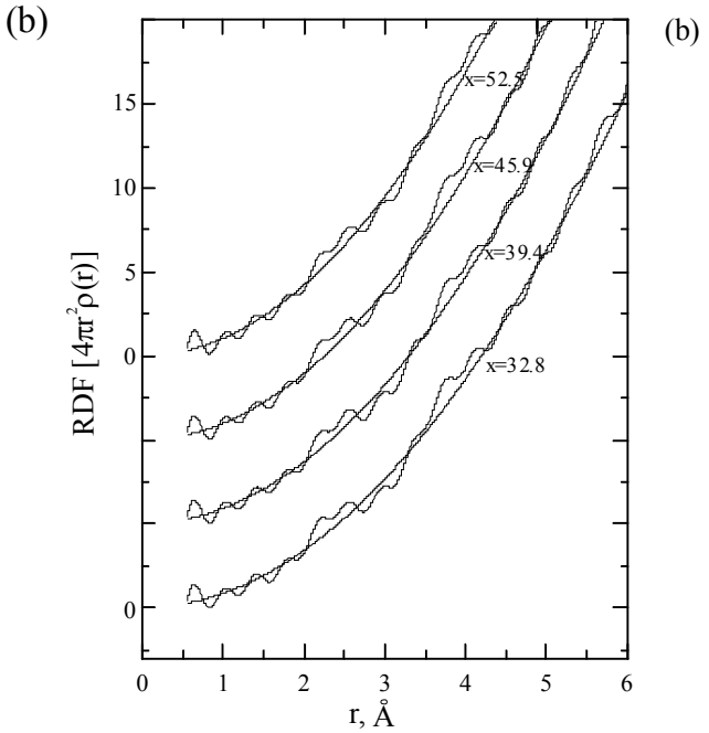
Fig. 4. Radial distribution functions of the atomic density of the glassy alloys of the \text{AgGaSe}_2+\text{GeSe}_2 \rightleftharpoons \text{AgGaS}_2+\text{GeSe}_2 system ( x – at% of Se).
