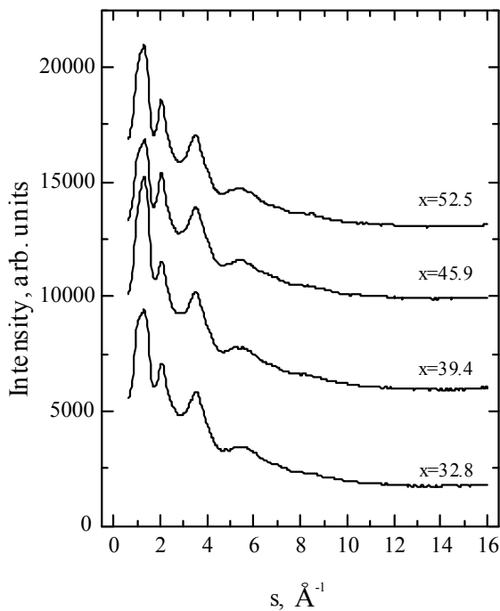
Fig. 3. X-ray scattering intensities of the glassy alloys of the \text{AgGaSe}_2+\text{GeSe}_2 \rightleftharpoons \text{AgGaS}_2+\text{GeSe}_2 system ( x – at% of Se).
