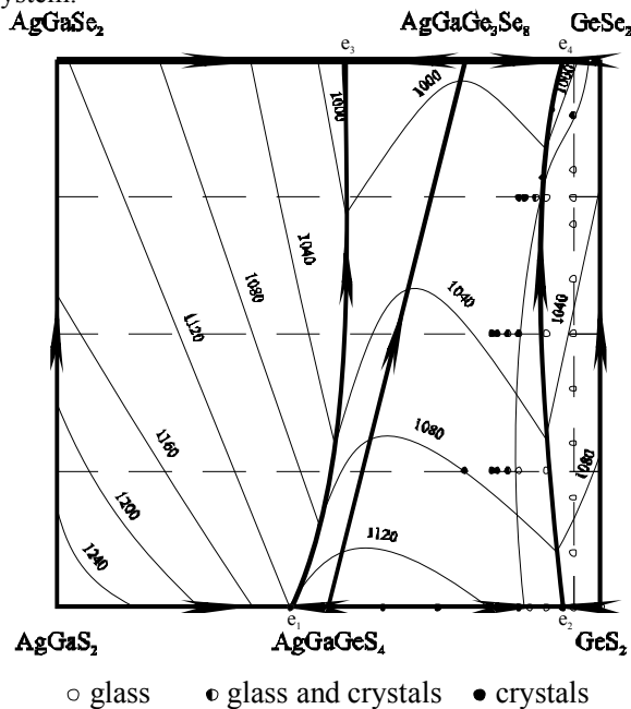
Fig. 2. Liquidus surface projection and the glass formation region of the \text{AgGaSe}_2 + \text{GeS}_2 \leftrightarrow \text{AgGaS}_2 + \text{GeSe}_2 system.
