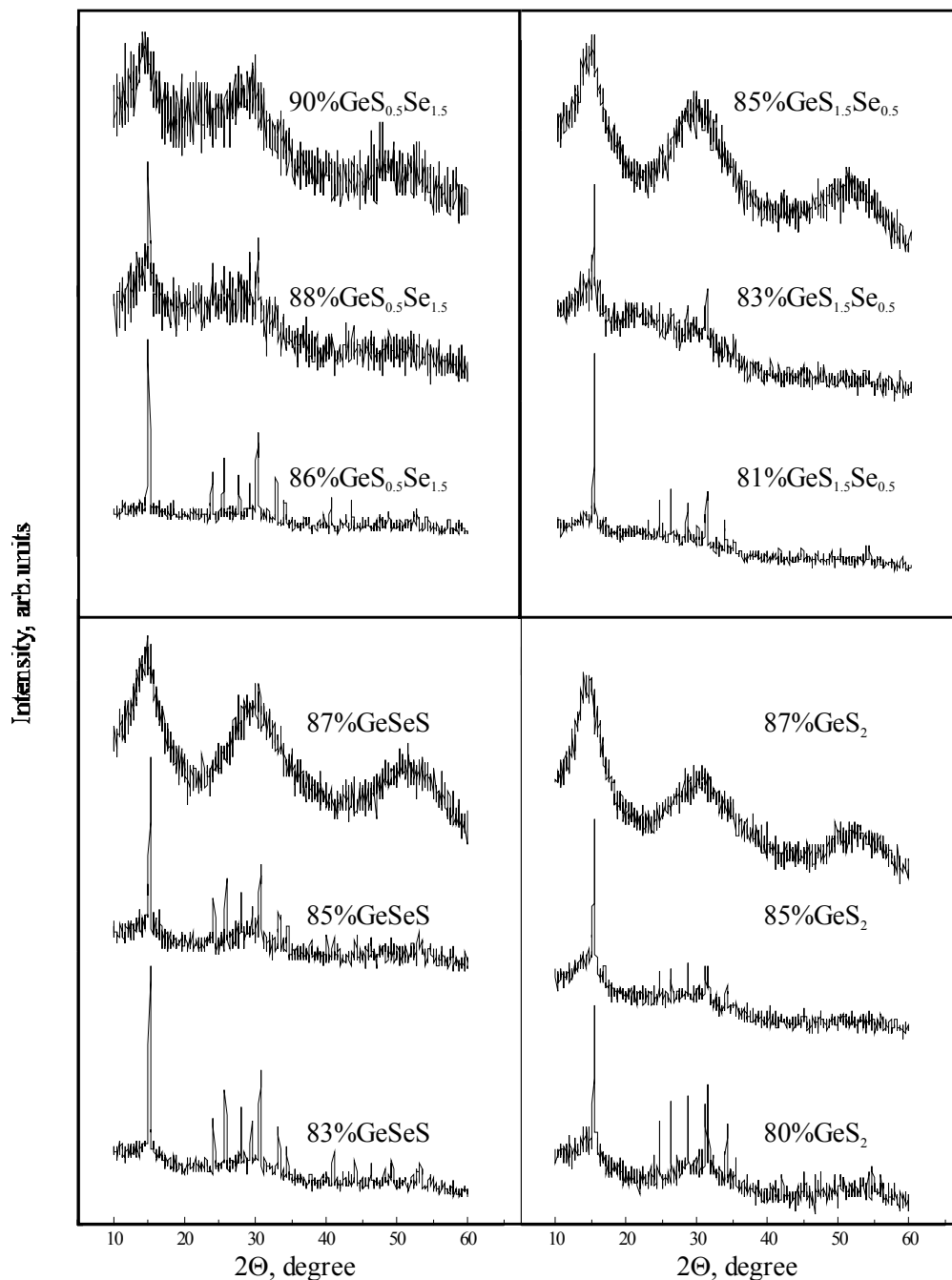
Fig. 1. Diffraction patterns of the alloys of the AgGaSe 2 +GeS 2 ↔AgGaS 2 +GeSe 2 system.
