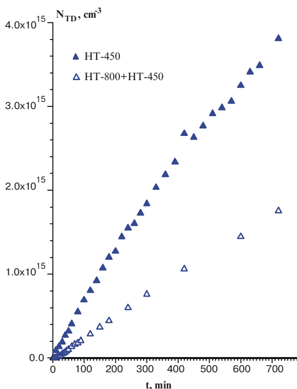
Fig.1. Dependence of thermodonor concentration on heat treatment time at 450 °C.
