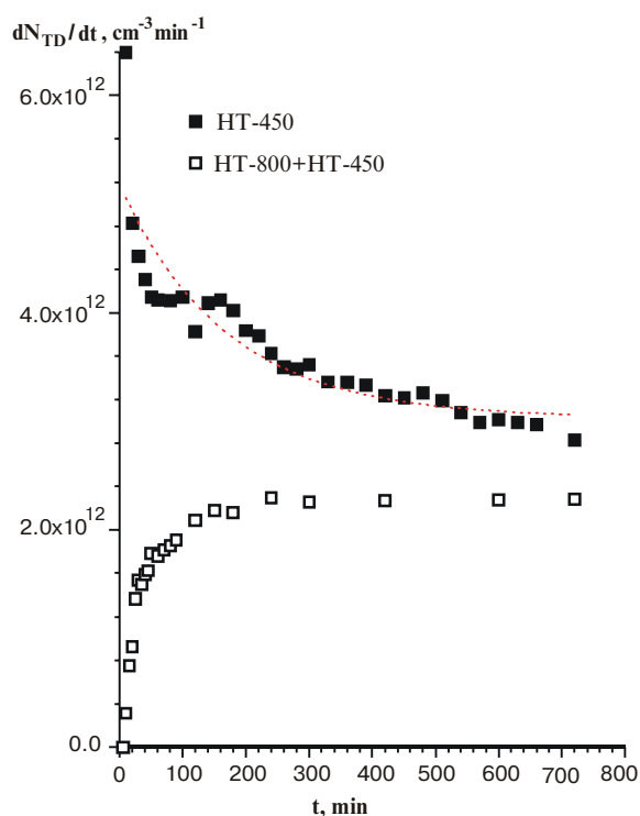
Fig.2. Dependence of thermodonor formation rate on heat treatment time at 450 °C.
