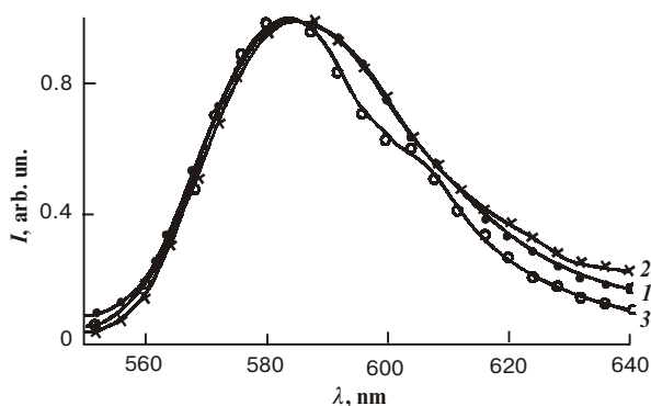
Fig. 5. PL spectra of ZnS:Mn single crystals – \lambda_{\text{exit}} = 396 nm, T = 77 K, C_{\text{Mn}} = 1 \cdot 10^{-2} g/g at a different degree of PD: \varepsilon = 0 (1), 1.57 (2); 1.78 % (3).
